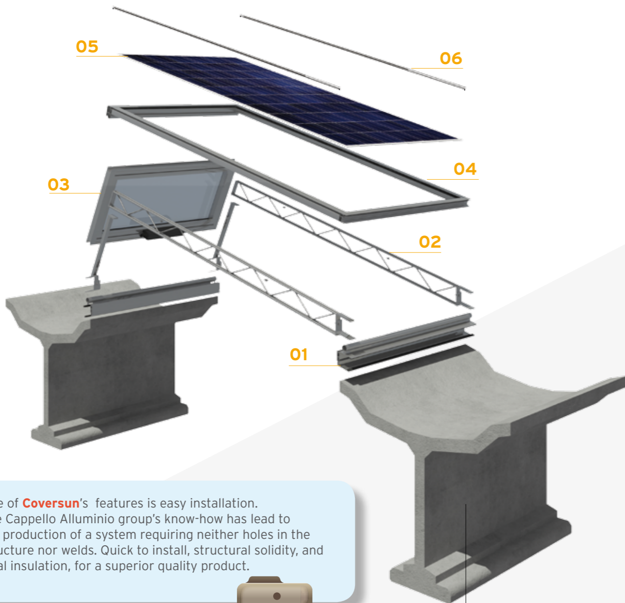
prestressed reinforced concrete Y-beam (or similar)
